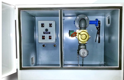
Remote Fill System
