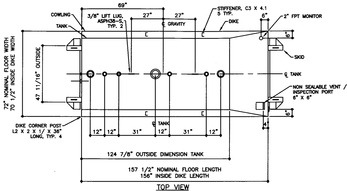
TOP VIEW
