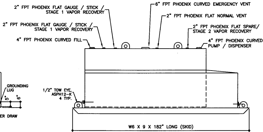
ELEVATION - SIDE VIEW
