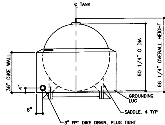
ELEVATION - END VIEW
