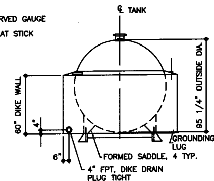
ELEVATION - END VIEW
