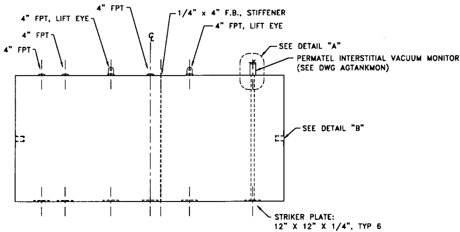
ELEVATION - SIDE VIEW
