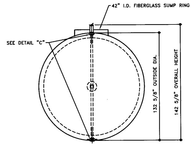
ELEVATION - END VIEW
