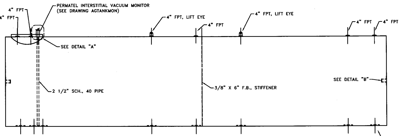
ELEVATION - SIDE VIEW
