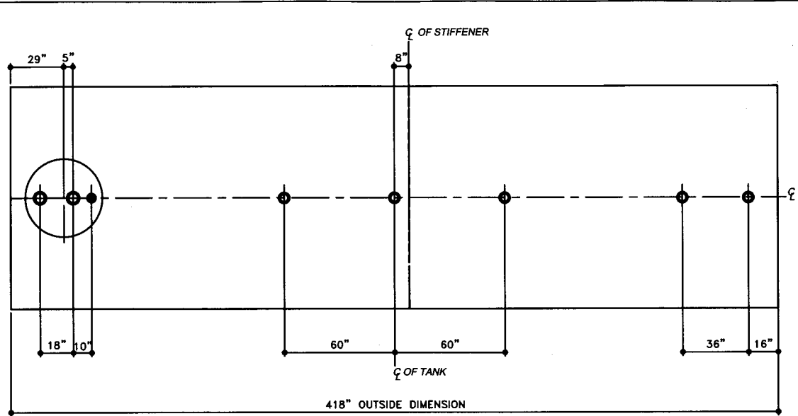
TOP VIEW
