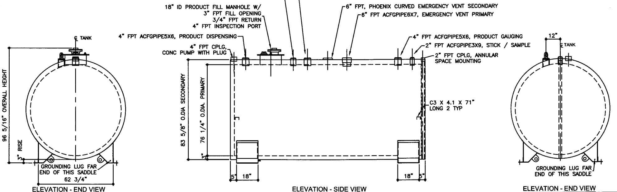
ELEVATION - SIDE VIEW
