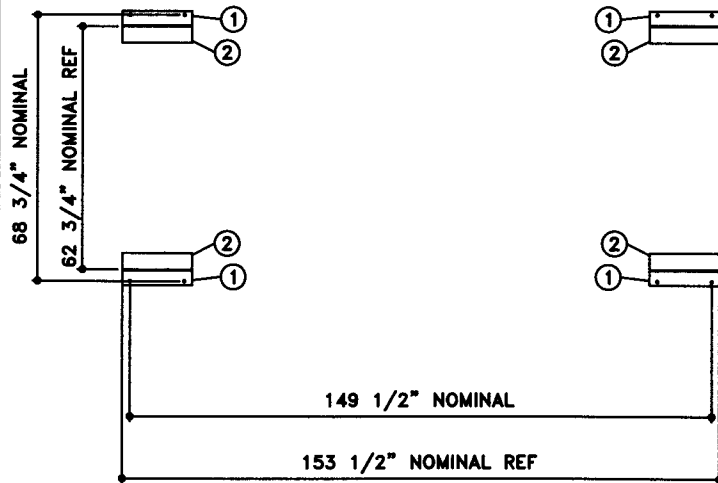
HOLDDOWN - TOP VIEW
