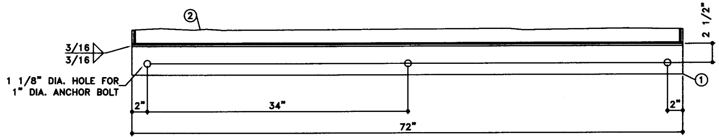
SECTION VIEW
