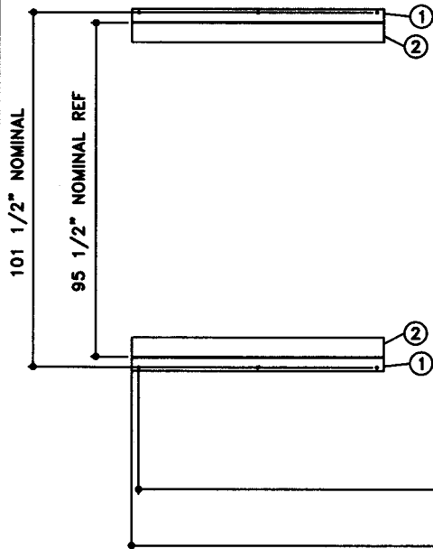
ELEVATION - END VIEW SEISMIC HOLD DOWN
