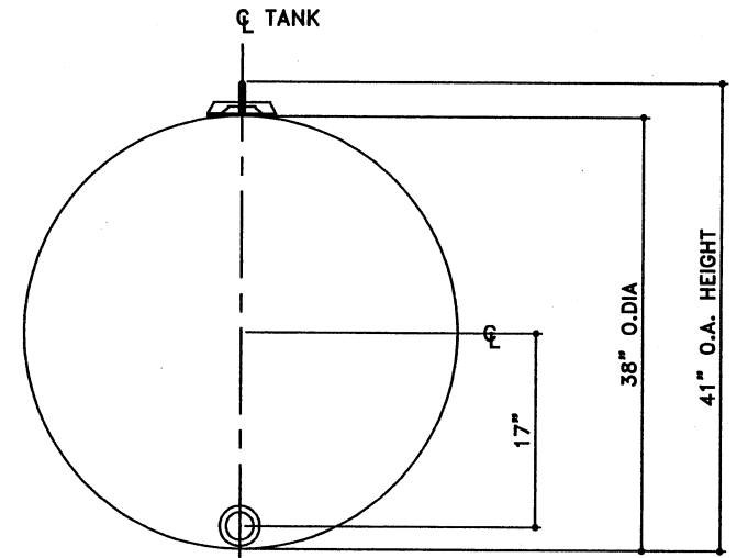
ELEVATION - END VIEW
