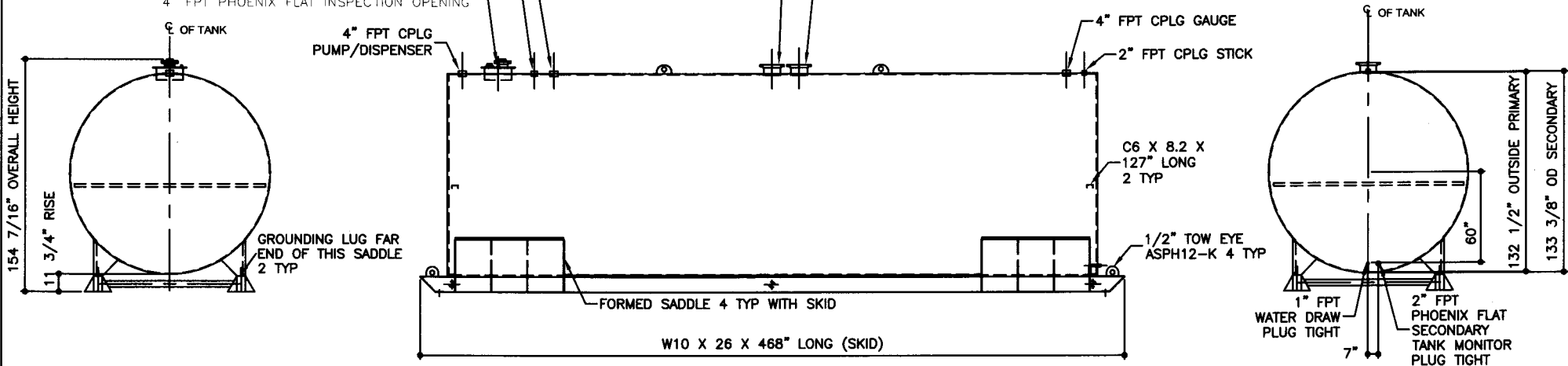
ELEVATION - END VIEW
