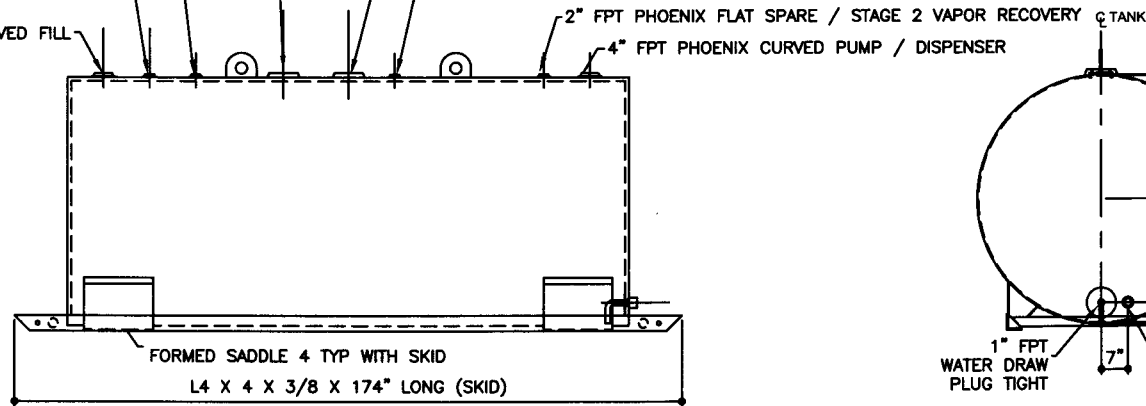
ELEVATION - SIDE VIEW
