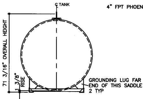
ELEVATION - END VIEW
