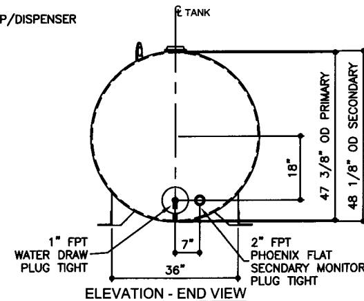
ELEVATION - END VIEW
