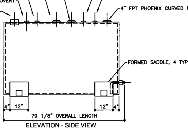
ELEVATION - SIDE VIEW
