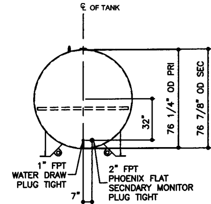
ELEVATION - END VIEW
